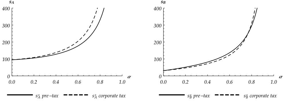
Panel B: Comparison of optimal s_A and s_B under decentral production and \tau_A > \tau_B
